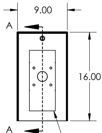
A8207-VE MK2 RECESSED MOUNT
