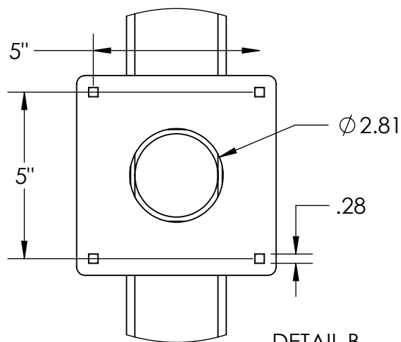
DETAIL B
