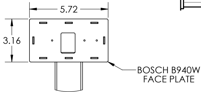
DETAIL A
